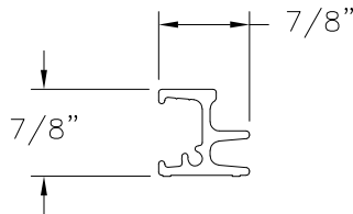
MEETING RAIL REINFORCEMENT (10635) ALUMINUM 6063-T5
