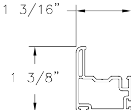
SASH STILE (9008) EXTRUDED RIGID PVC
