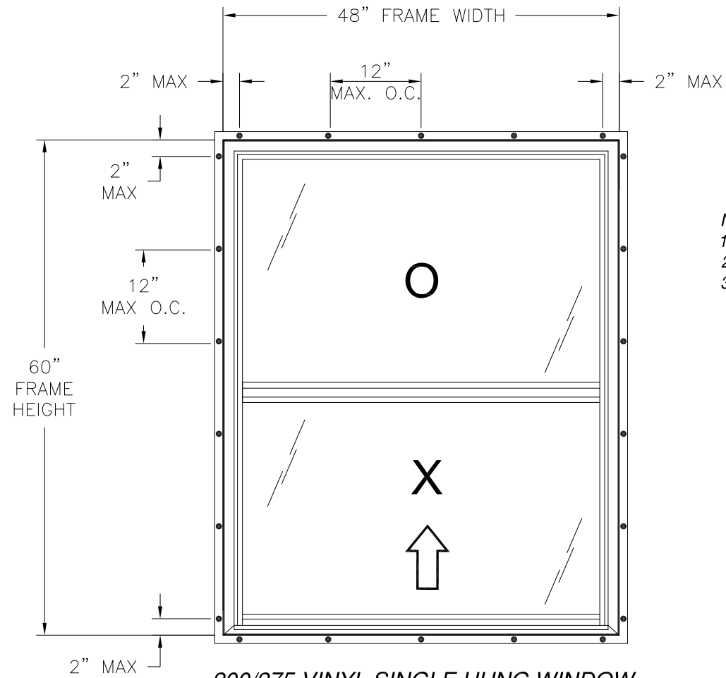
200/275 VINYL SINGLE HUNG WINDOW EXTERIOR VIEW
